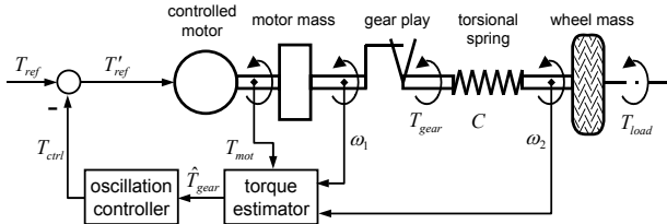
Fig. 4. Control structure
